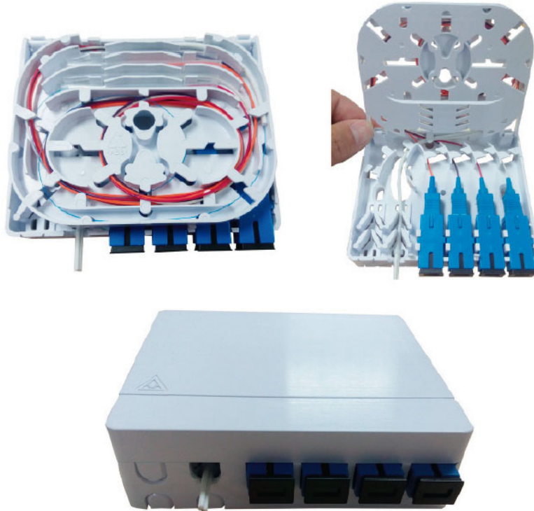
Fig. 1: FTTH Fiber Socket
